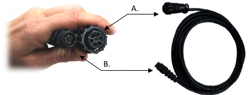
A. Round AMP Connector B. 5-pin Female Switchcraft Connector
